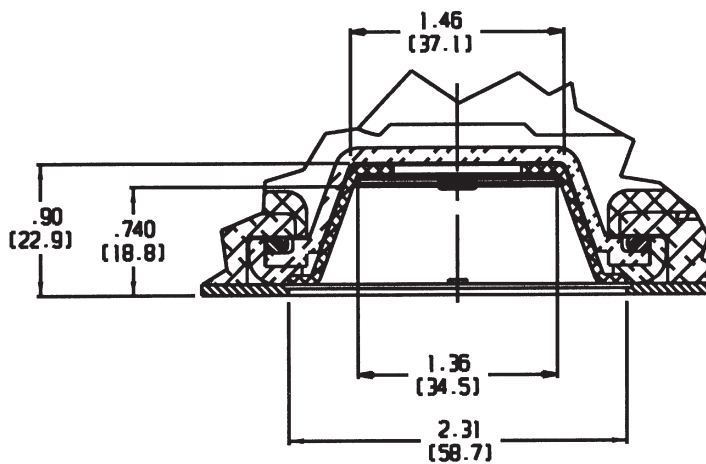
Cross Section of Port 端口的横截面
